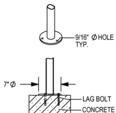
SURFACE MOUNT (SM)
