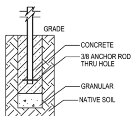
IN GROUND MOUNT (IG)
