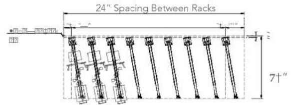
10° Layout Plan
